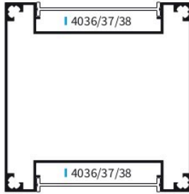
4035 Stub za ogradu 100x100 L Louvre 100x100x1,5 mm
